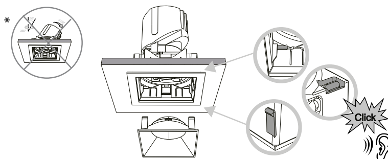
Reflector + Anti-glare ring
